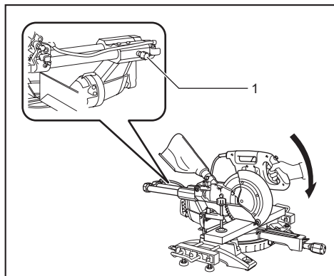
► 1. Locking screw
